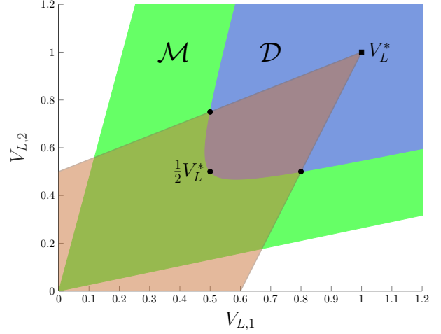
Fig. 7. A plot of the voltage domain for a power grid with two load nodes. The blue area corresponds to the set \mathcal{D} of long-term voltage stable operating points. The brown area indicates the operating points corresponding to a nonnegative power demand. The green area corresponds to the vectors in \mathcal{M} , which contains the set \text{cl}(\mathcal{D}) . The black operating points correspond to the black power demands in Figure 8.
